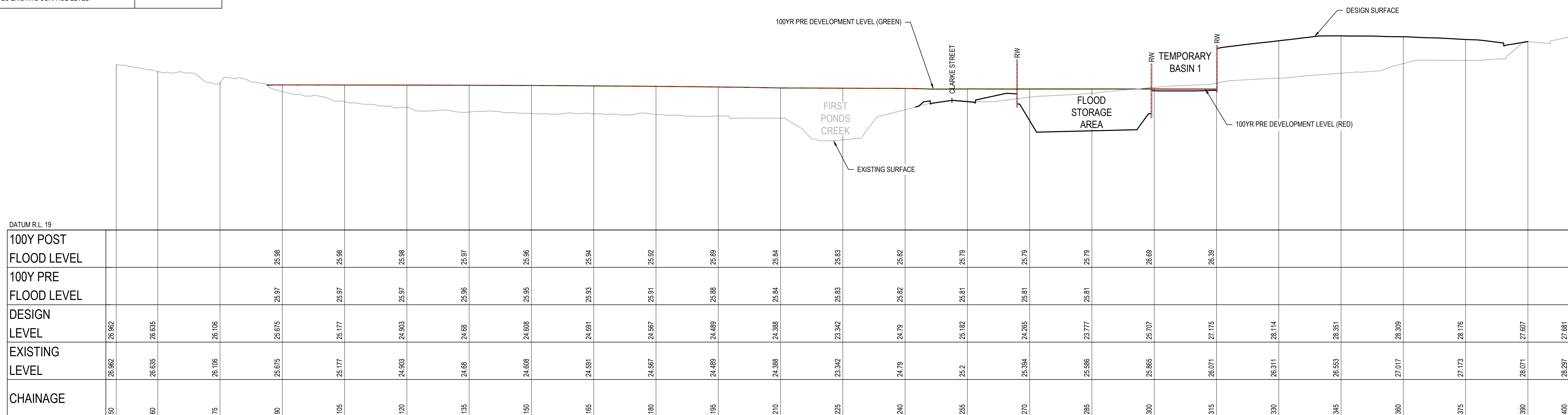
SECT 1-2024.68 SCALE 1:500 (H) SCALE 1:100 (V)
